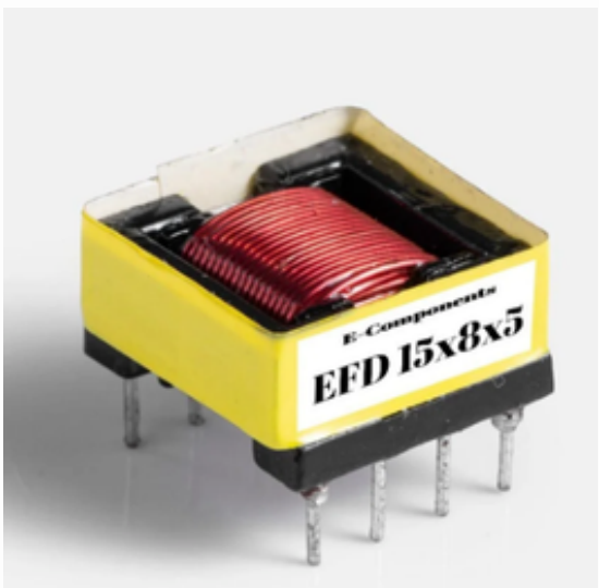
EFD15x8x5 8P "H"
