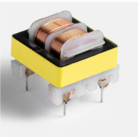
EE25x13x7 4P "H"
